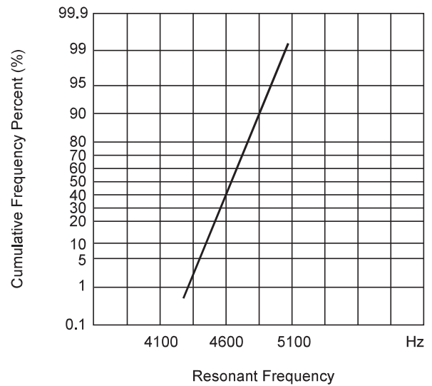
(4) Resonant Frequency
