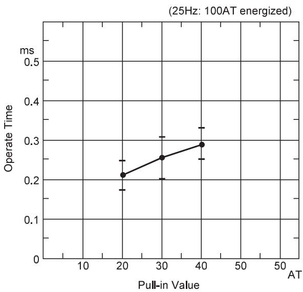
(1) Operate Time
