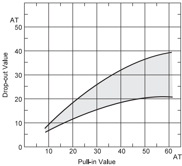
(1) Pull-in Value vs. Drop-out Value
