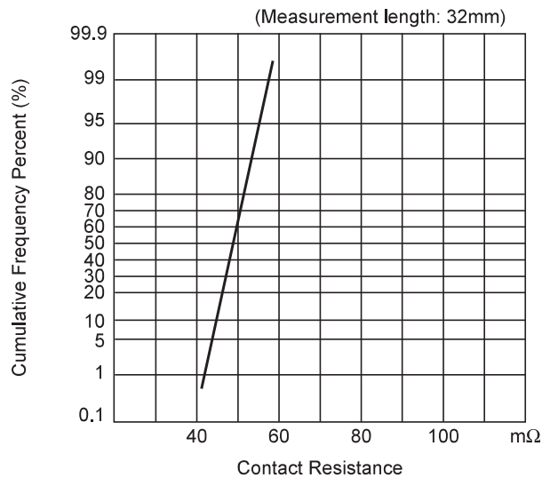
(2) Contact Resistance
