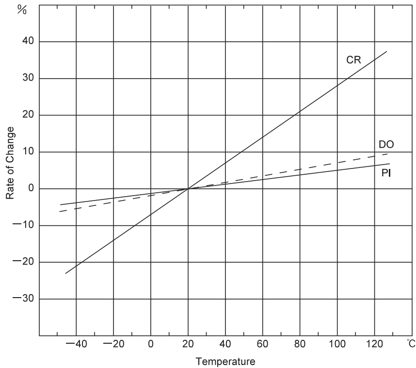
(1) Temperature Characteristics
